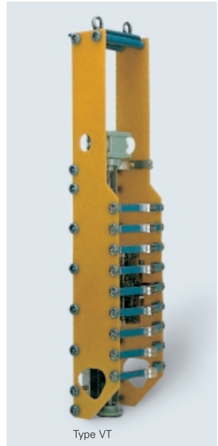
Fig. 47: Gas-insulated on-load tap changer
