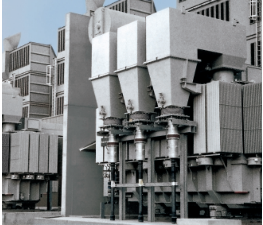
Fig. 14: Transformers with oil-filled HV cable boxes
