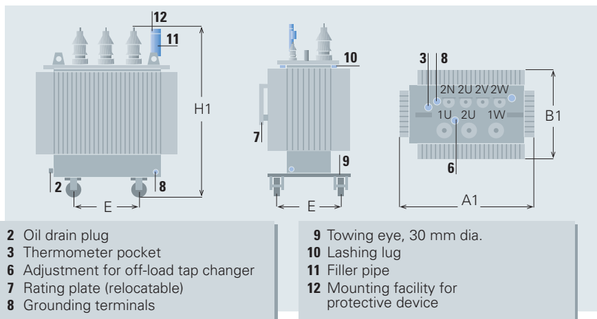
Fig. 24: TUMETIC distribution transformer (sealed tank)
