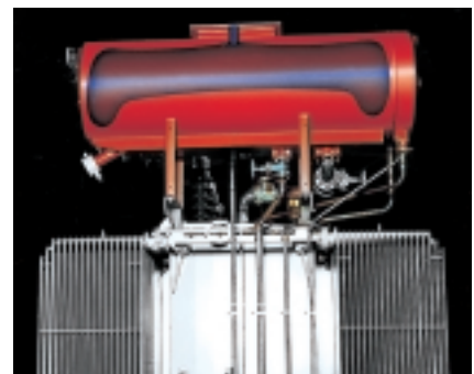
Fig. 9: Practically maintenancefree: transformer with the TUPROTECT air-sealing system built into the conservator
