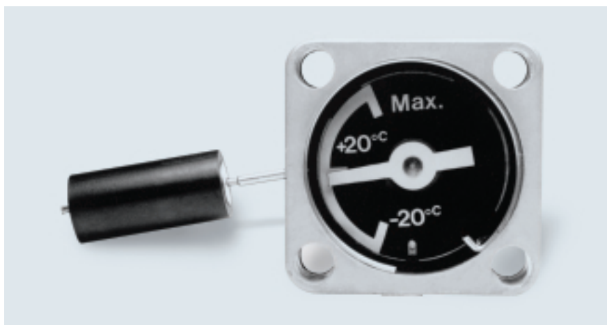
Fig. 18: Magnetic oil-level indicator
